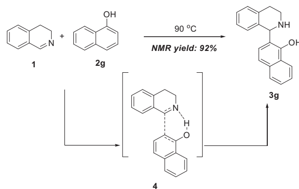
Scheme 2. Hydrogen-bonding assisted C–C bond formation.
