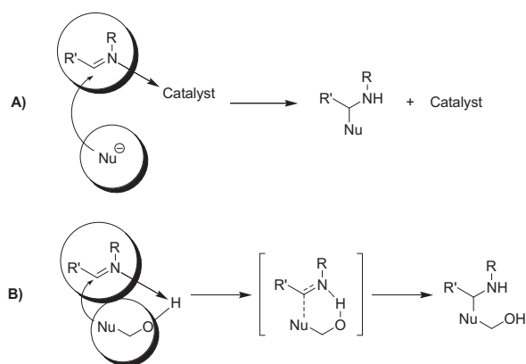
Scheme 1. Typical Lewis or Brønsted acid catalyzed system (Path A) versus the proposed self-catalytic system (Path B).
